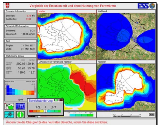
Figures 4,5 : district heating scenario showing blocks connected in white; comparative analysis of the model results with and without a possible district heating scheme.
